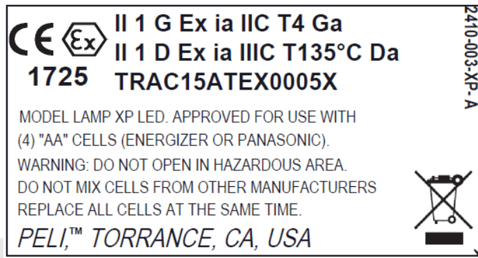
Marking plate for MSA Lamp XP LED by Peli
