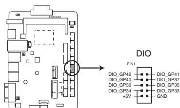
Apollo Lake Digital I/O connector
