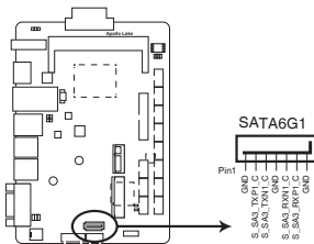
Apollo Lake SATA 6.0Gb/s connector
