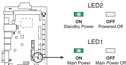
Apollo Lake Onboard LEDs
