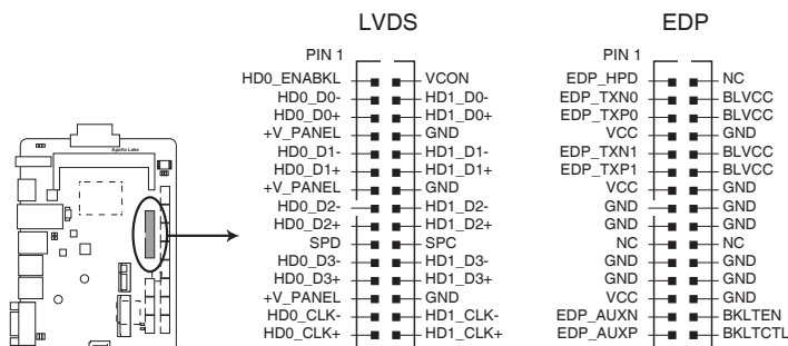
Apollo Lake LVDS/EDP connector
