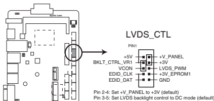
Apollo Lake LVDS panel voltage selection
