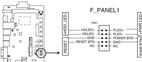
Apollo Lake System panel connector
