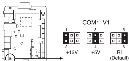
Apollo Lake COM1 RI/+5V/+12V selection
