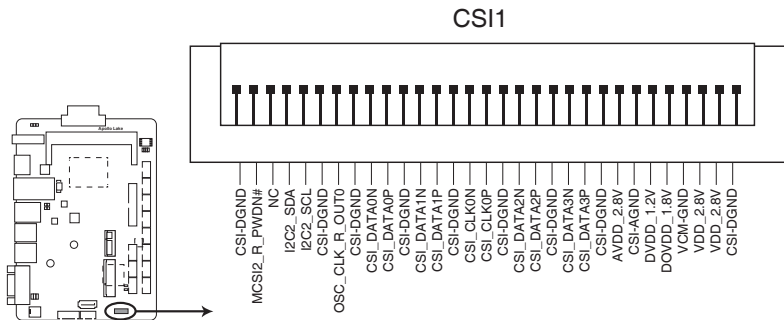
Apollo Lake Camera Serial Interface connector
