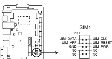
Apollo Lake Internal SIM card connector
