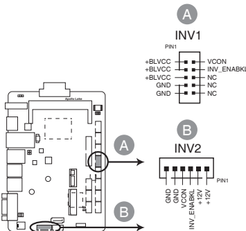
Apollo Lake Inverter connectors
