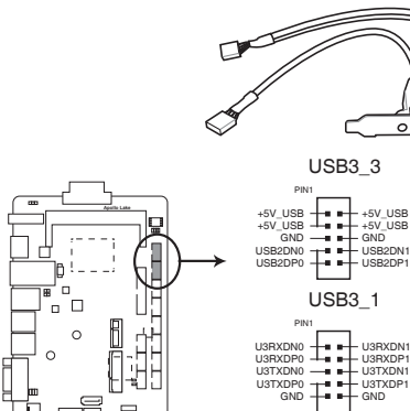
Apollo Lake USB3.0 connectors
