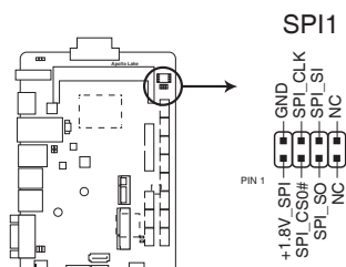
Apollo Lake BIOS programming connector for Aaeon
