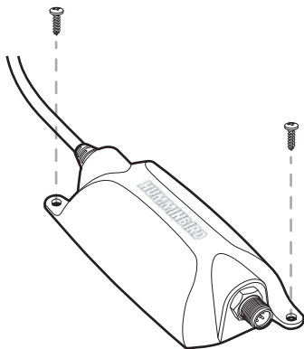
Installing the NMEA 2000® Module
