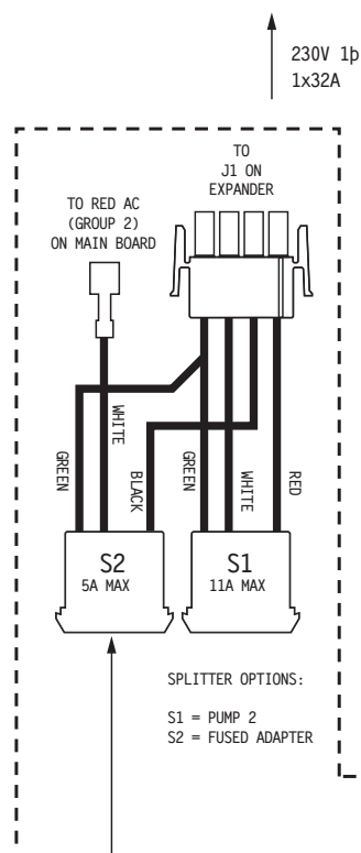
SINGLE SERVICE 230V 1p / 1x32A, DUAL SERVICE 230V 2x1p / 3x16A, THREE-SERVICE 230V 3p / 3x16A
