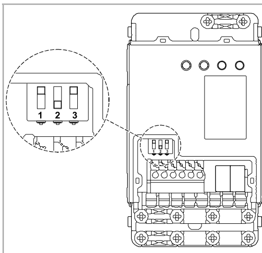
Afb. 7: DIP-switches
