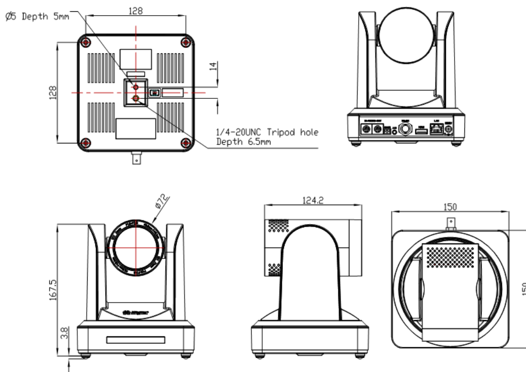
Figure 2.2 Camera dimension
