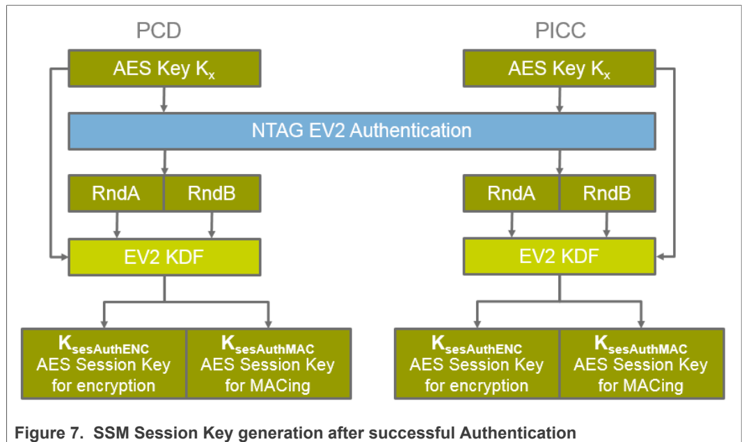
Figure 7. SSM Session Key generation after successful Authentication
