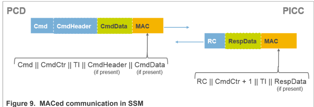
Figure 9. MACed communication in SSM
