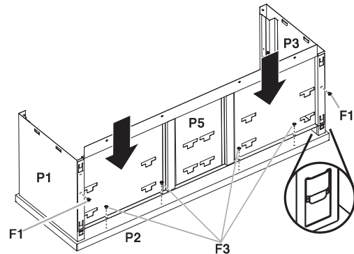
F1 #10-24 x 1/4" long Phillips-head screw (2) F3 #8 x 1/2" long Phillips-head screw (4)
