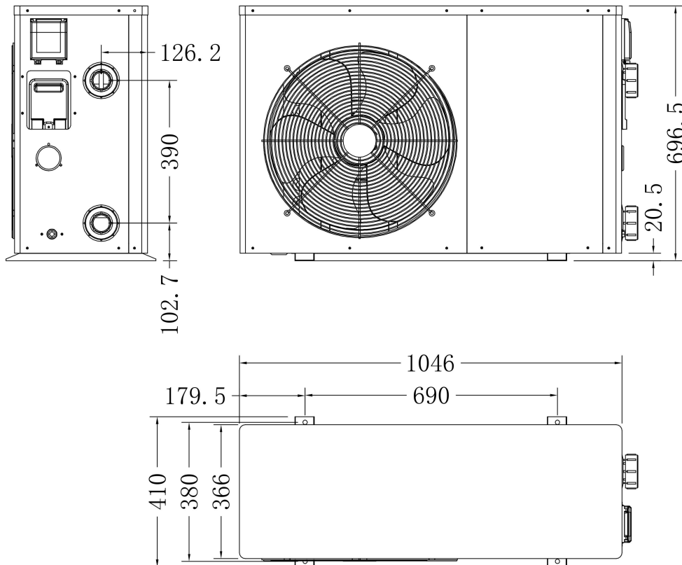
Hydro-S Inverter 12/16
