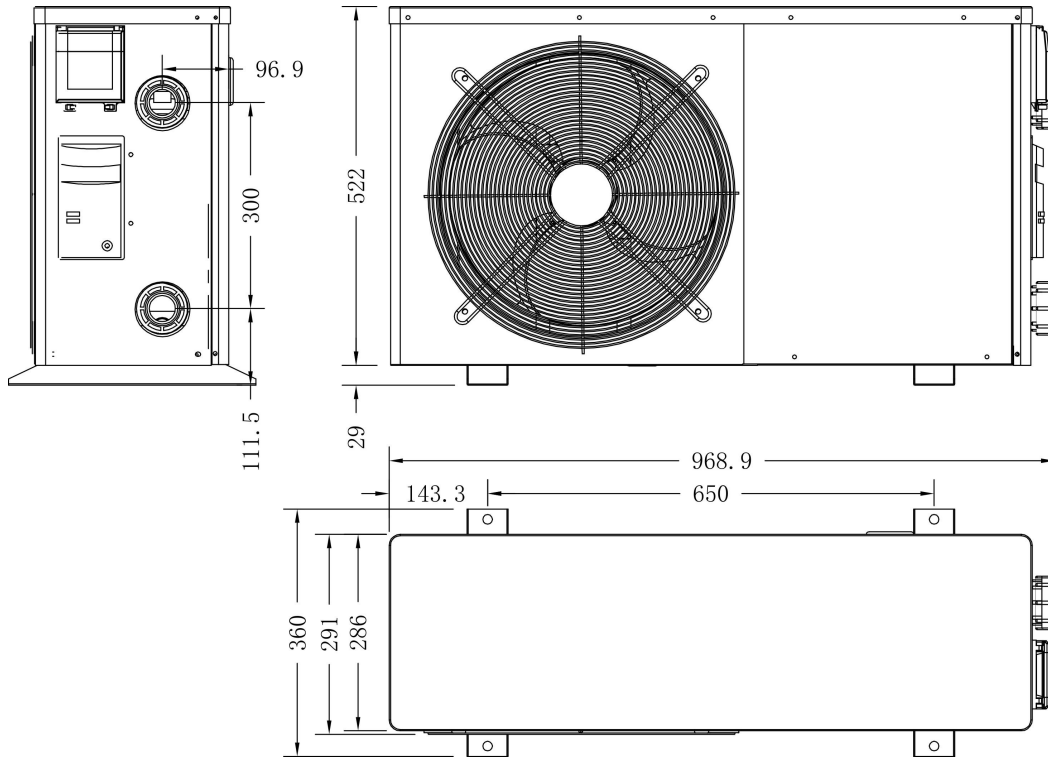
Hydro-S Inverter 5/6/9
