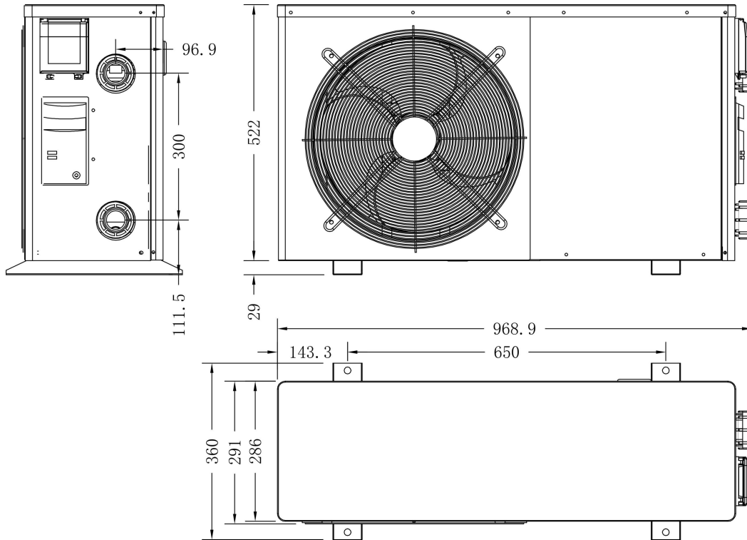
Hydro-S Inverter 5/6/9
