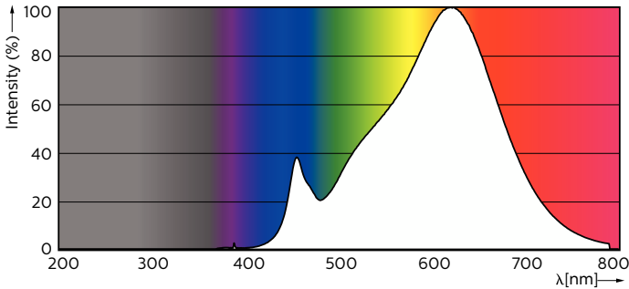
Spectral Power Distribution Colour - MAS LED spot VLE DT 4.9-50W GU10 927 36D
