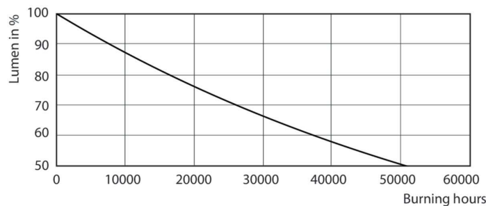
Lumen Maintenance Diagram - MAS LED spot VLE D 4.9-50W GU10 940 36D
