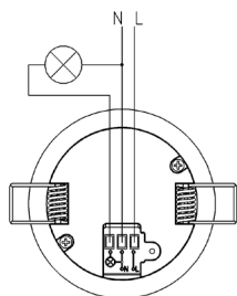
Connection-wire diagram
