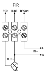
Connection-wire diagram
