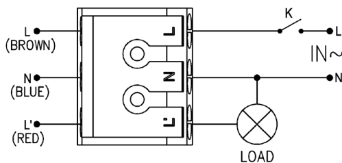
Connection-wire diagram
