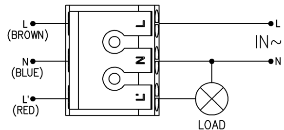
Connection-wire diagram
