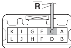
0912-303 POWER WINDOW SUBSWITCH (RF)
