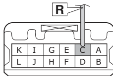
0912-303 POWER WINDOW SUBSWITCH (LF)
