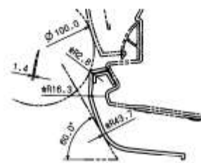
SEC. C-C
