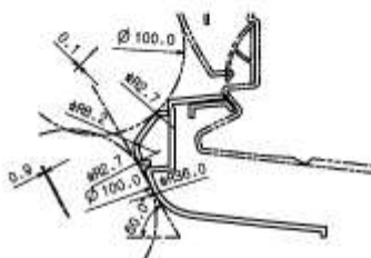
SEC. B-B
