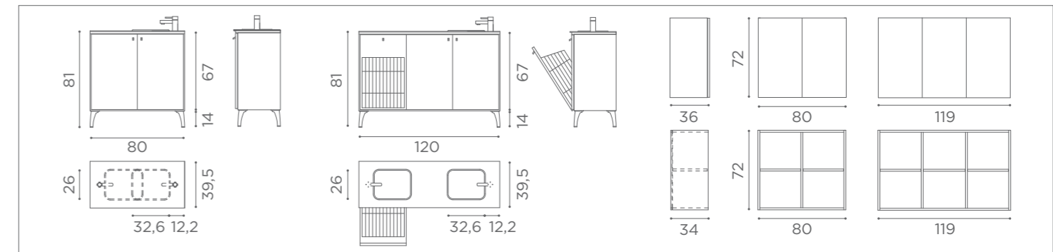
ALUMINIUM FEET
