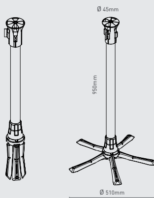
Pfosten | Post
