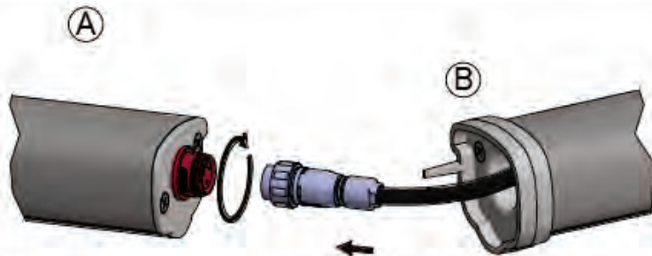
Plug Male & Female Connector Together & Twist to Seal
