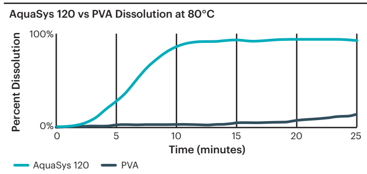
Figure 1: Dissolution Kinetics of AquaSys 120 and PVA
