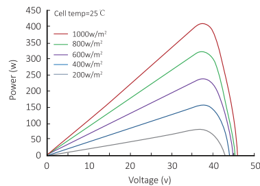
Power-Voltage Curve (LR4-66HPH-405M)
