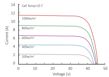
Current-Voltage Curve (LR4-66HPH-405M)
