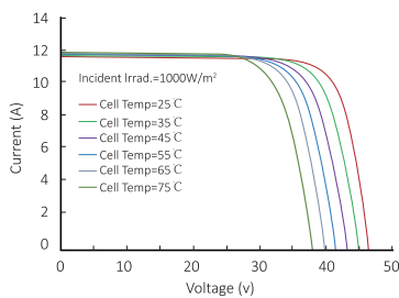
Current-Voltage Curve (LR4-66HPH-405M)
