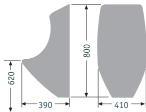
Model eco
