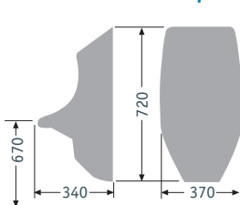
Model compact
