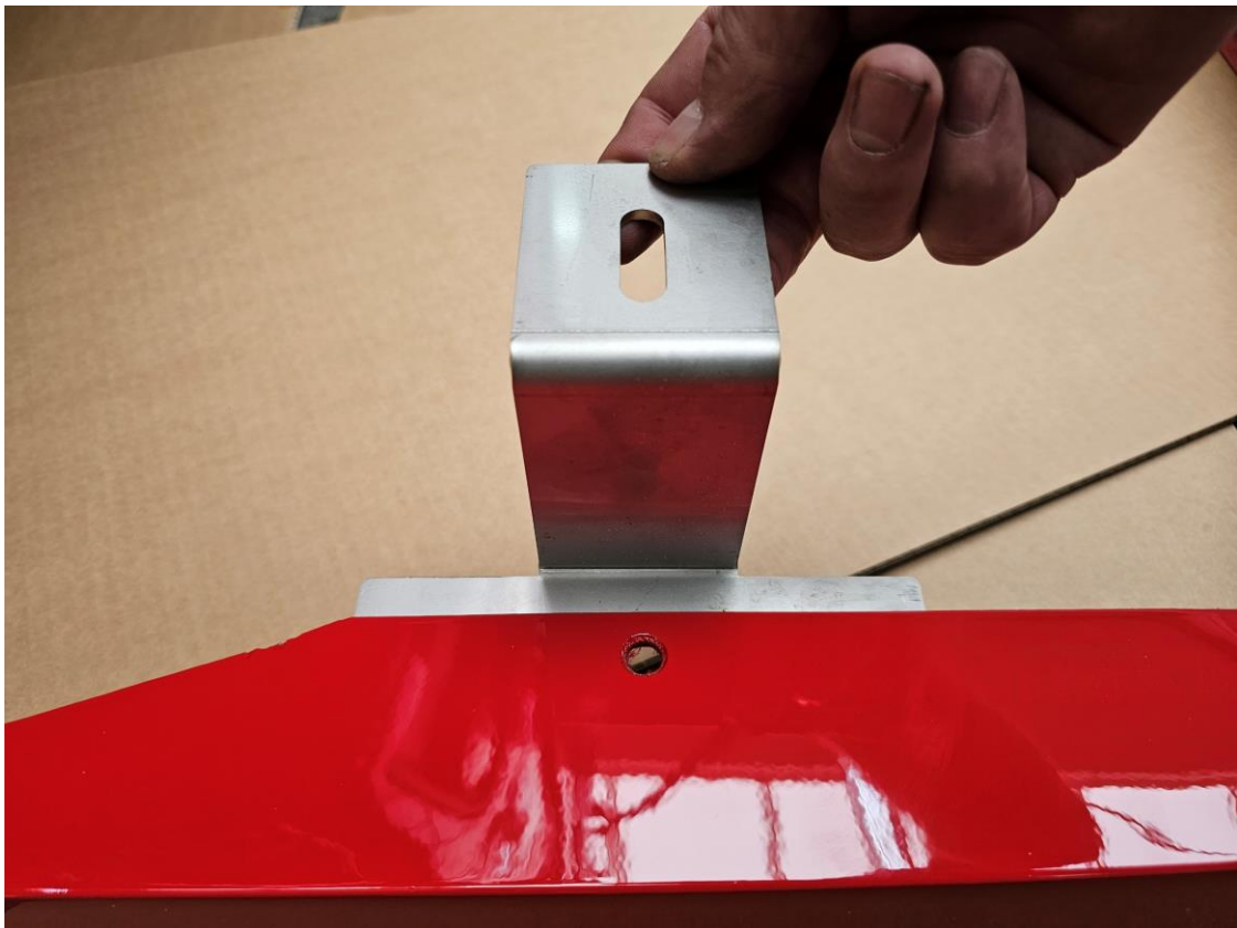
SIDE MOUNTING BRACKET
