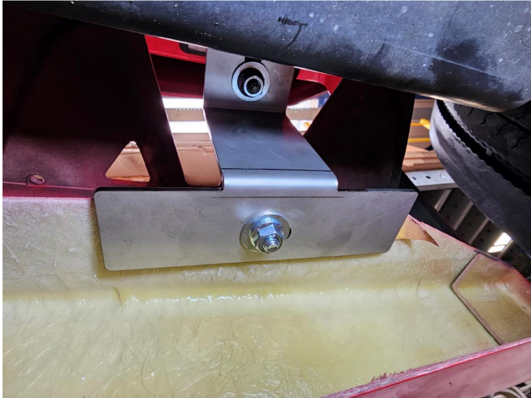
BOTTOM VIEW SIDE MOUNTING BRACKET
