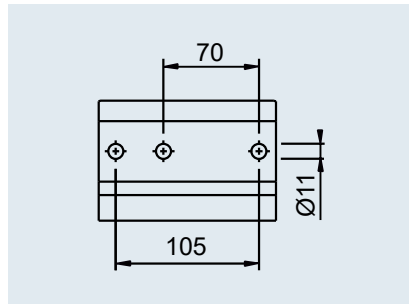
Jockey wheel flange
