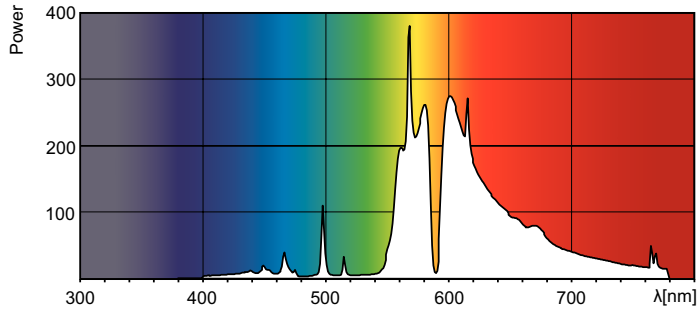
LDPO_SONTHORT_0005-Spectral power distribution Colour
