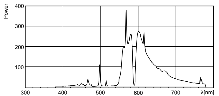
LDPB_SONTHORT_0005-Spectral power distribution B/W
