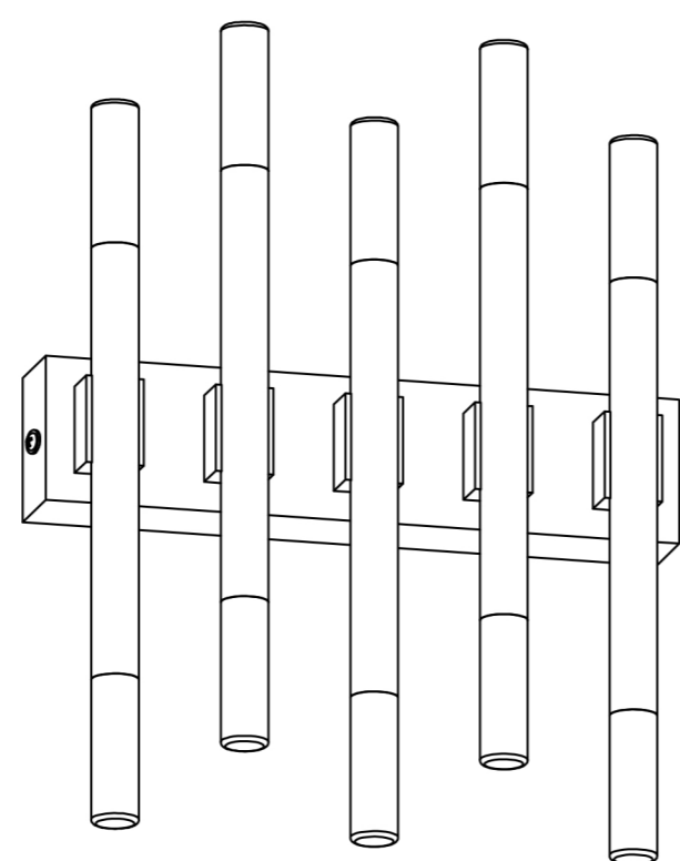
STIXX 5 L300×W220×H53(mm) LED-10×1W
