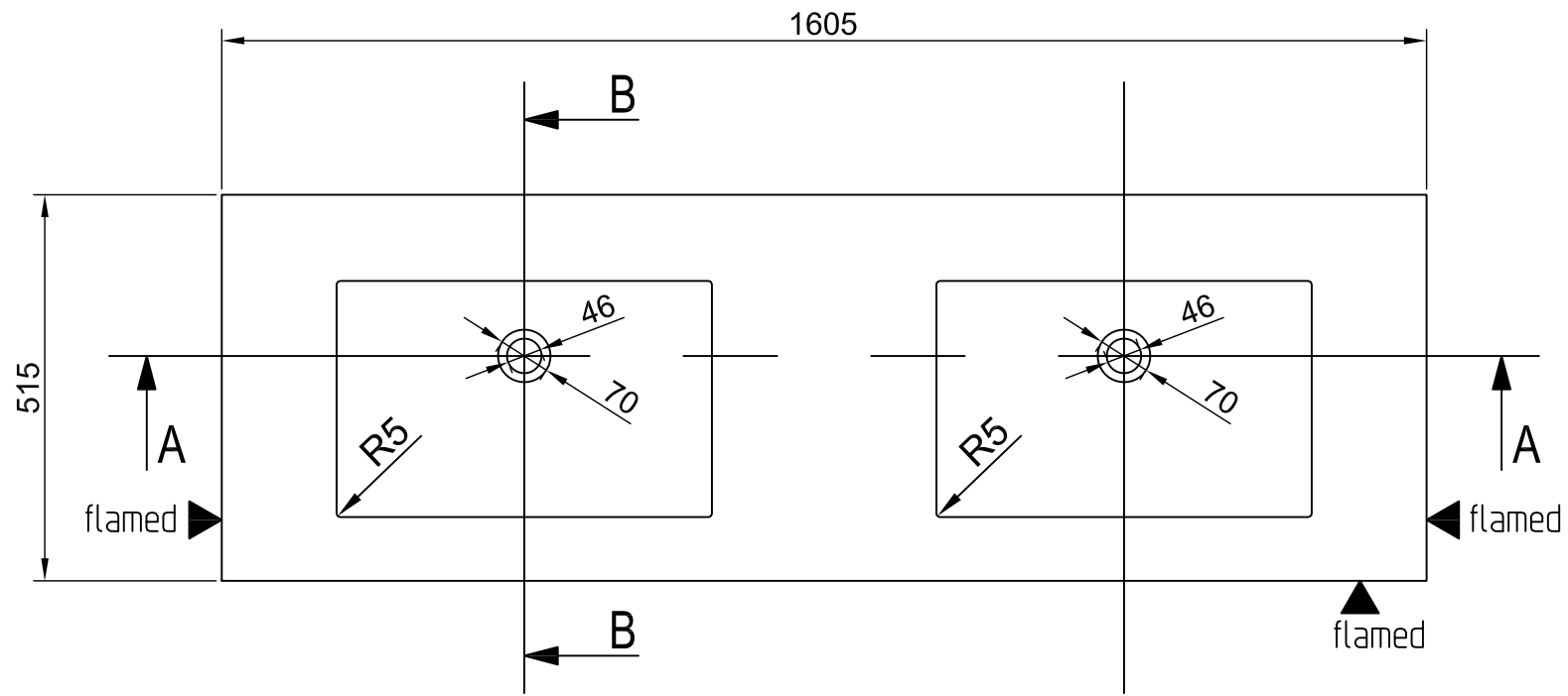
TOP VIEW
