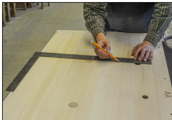
Illustration 16 - Mark Sostenuto pitman hole
