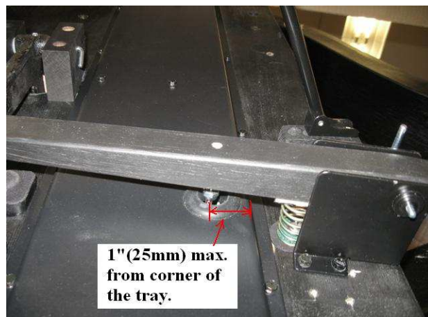
Illustration 74A – Max. distance for threaded rod
