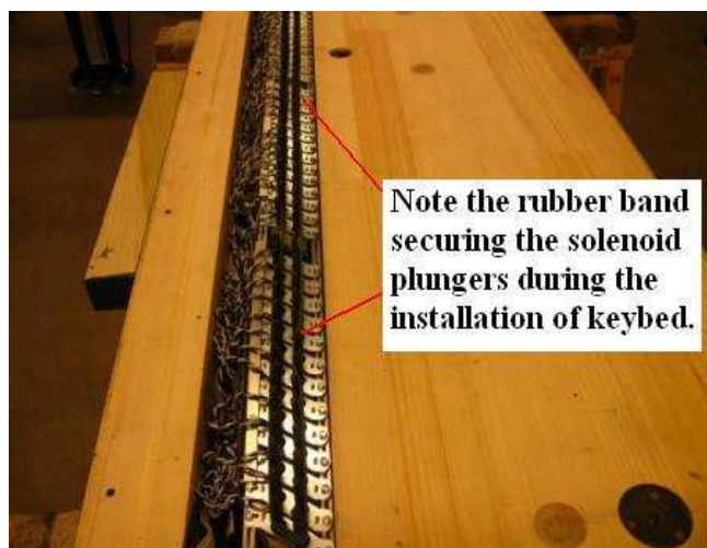
Illustration 142 – Securing key solenoid plunger with rubber band
