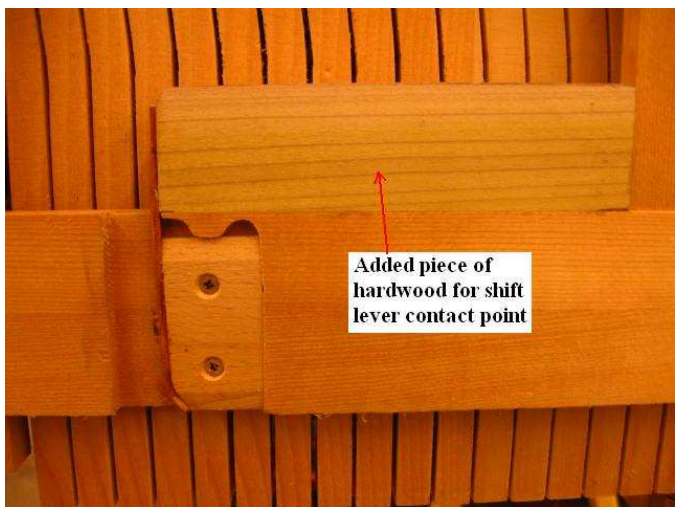
Illustration 2 – After adding hardwood
