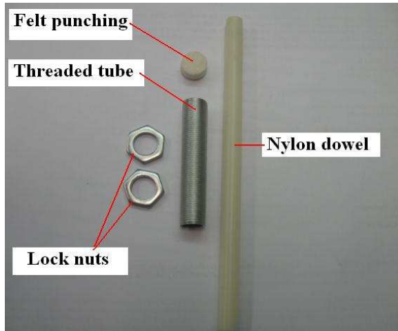
Illustration 1 – Steinway Sost. Kit
