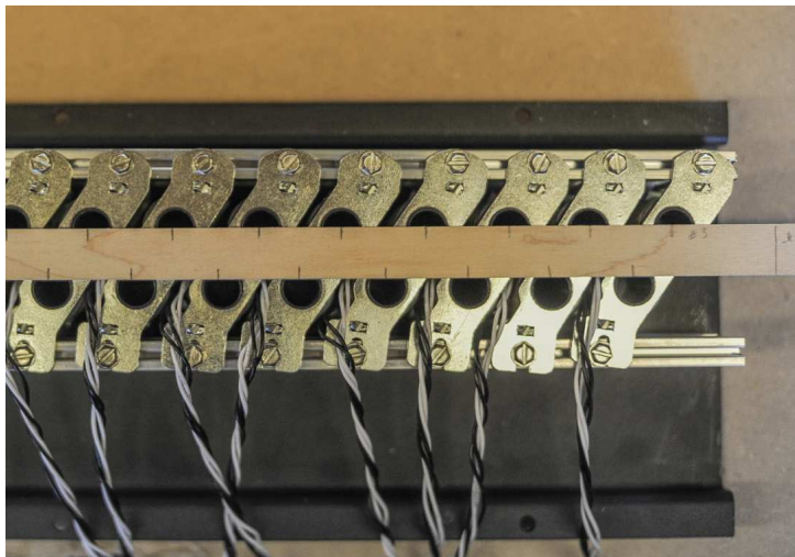
Illustration 122 - Use scale stick to locate solenoids
