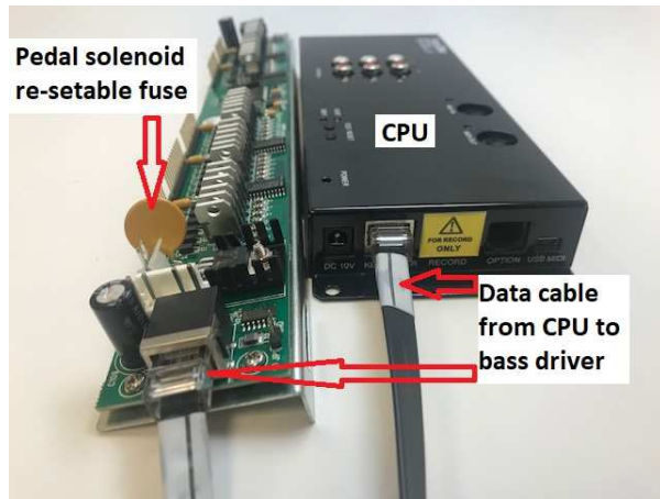
Illustration 130 - Connecting data
