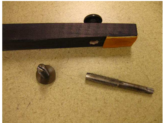
Illustration 108 - Glide stop installed
