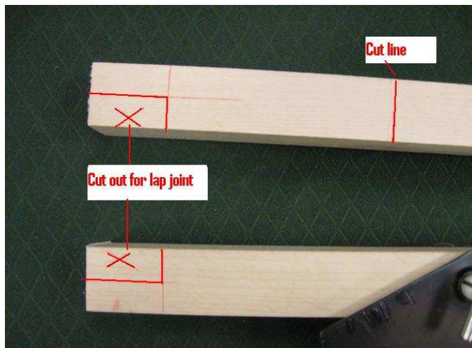
Illustration 103 - Sostenuto lever lap joint
