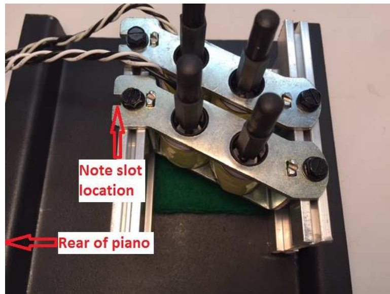
Illustration 20 – PD low profile solenoid rail systems
