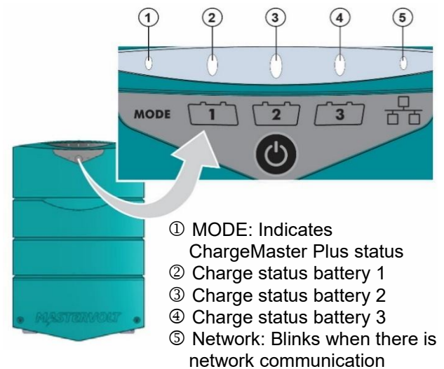
Figure 5: ChargeMaster Plus status LEDs
