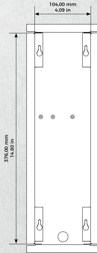
Flush-mounting housing (backbox)
