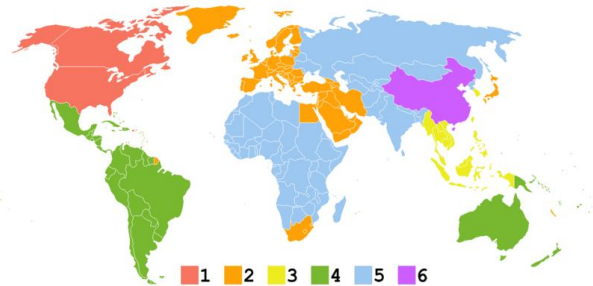
DVD regions
