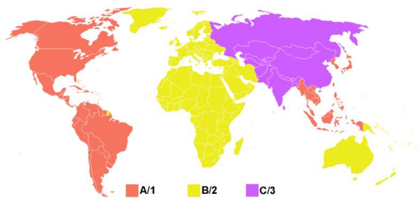
Blu-ray zones
