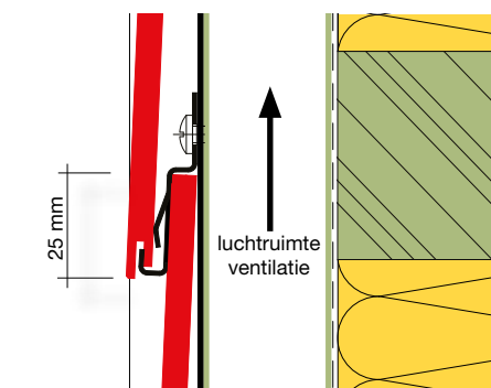
OVERLAP VAN DE POTDEKSELPLANKEN/SIDINGS
