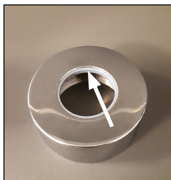
Step 4 Remove the nut from the old spout and ensure that the plastic bush remains in the nut.
