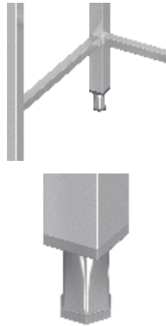
Welded frame. Legs made of stainless steel tube 40x40 mm. Frame made of stainless steel tube 25x25 mm
