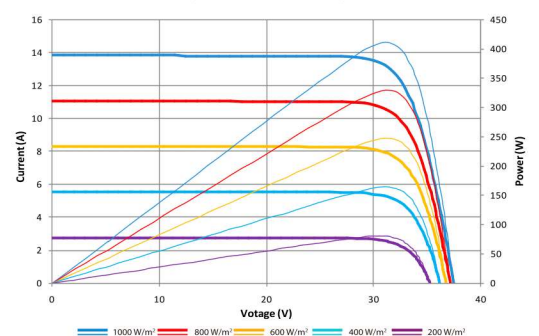
Current-Voltage & Power-Voltage Curve (410)
