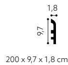
MD236 mat MD236P satin (RAL9003)
