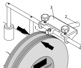
Trimming device, order no. 8949 0713
