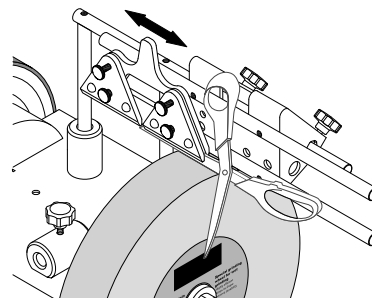
Device for scissors (with 100) 160, order no. 8949 0710
