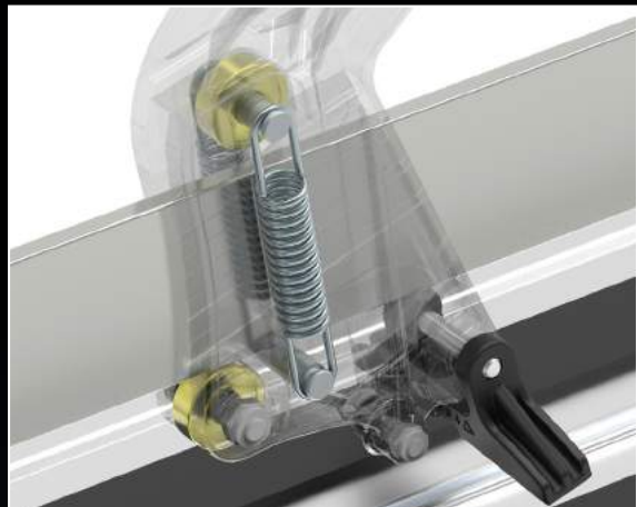
CARRIAGE The carriage in aluminium is equipped with two ball-bearings for a perfect sliding and top precision.
