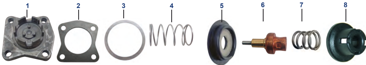
2, 3 CYL, V4 LOOPCHARGED (1992-00)
