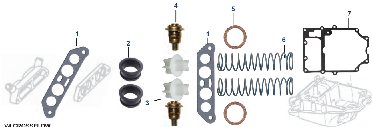
V4 CROSSFLOW
