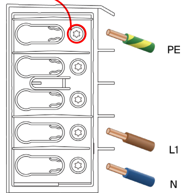
TN/TT 1-phase (230V)
