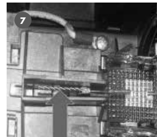
Make sure the contact wire is straight and not twisted before closing the fitting
