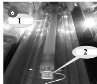
When replacing the lamp, make sure the glass vacuum seal (1) points away from the reflector and the getter (2) is on the ballast side
