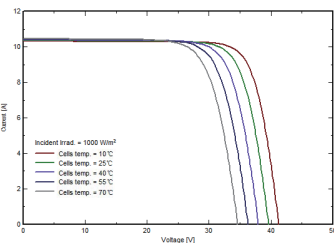
I-V Curve at different temperature (SPP320M60)
