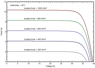
I-V Curve at different irradiation (SPP320M60)
