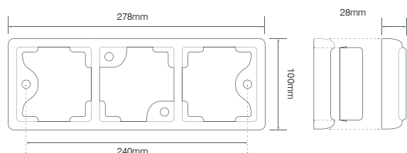
Triple lamp version 100-serie
