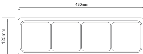
Quad lamp version 100-series
