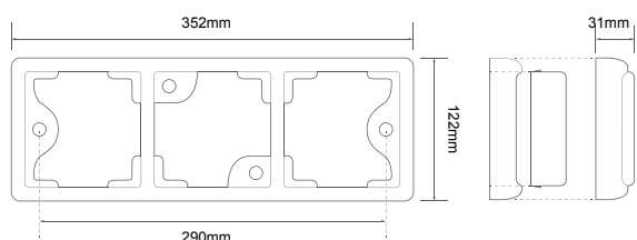
Triple lamp version 125-serie
