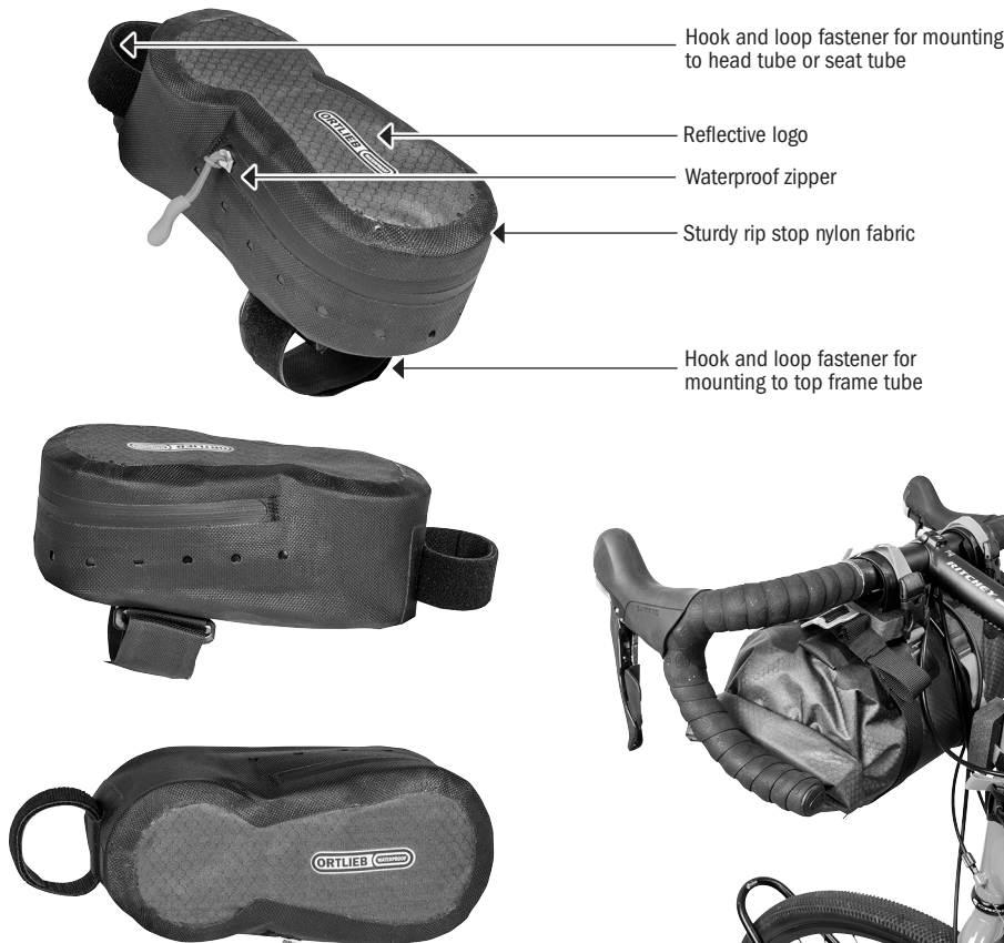
Example: Cockpit-Pack mounted to frame (Frame-Pack and Handlebar-Pack not included)
