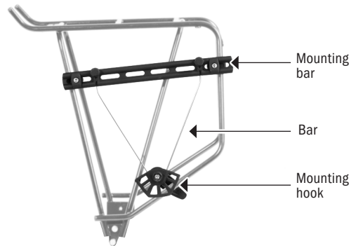
QL3/QL3.1 mounting components (incl.)
