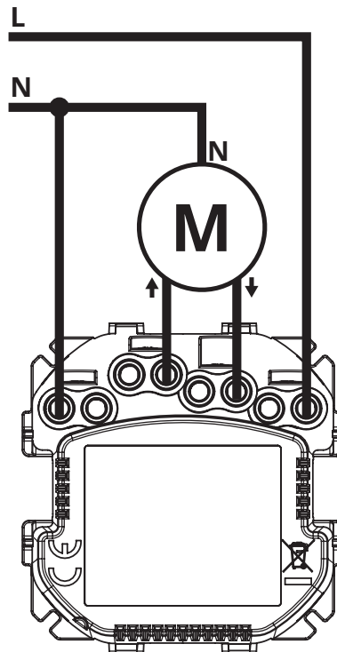
Diagram 1: Example connection with roller blind motor
