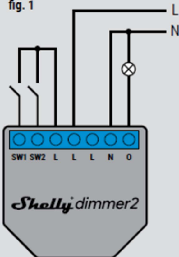
Standard wiring with neutral
