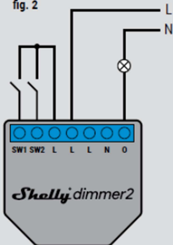
No neutral wiring*
