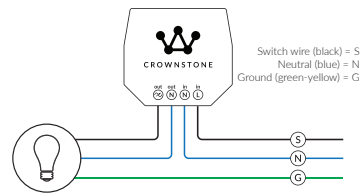
C) Built-in Crownstone connection diagram. Wire colors may be different in your situation. Ground wire could be missing.
