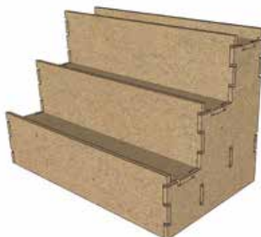
460.483.020 Basic box bottle stairs, 4mm MDF Size 220x150x130 mm
